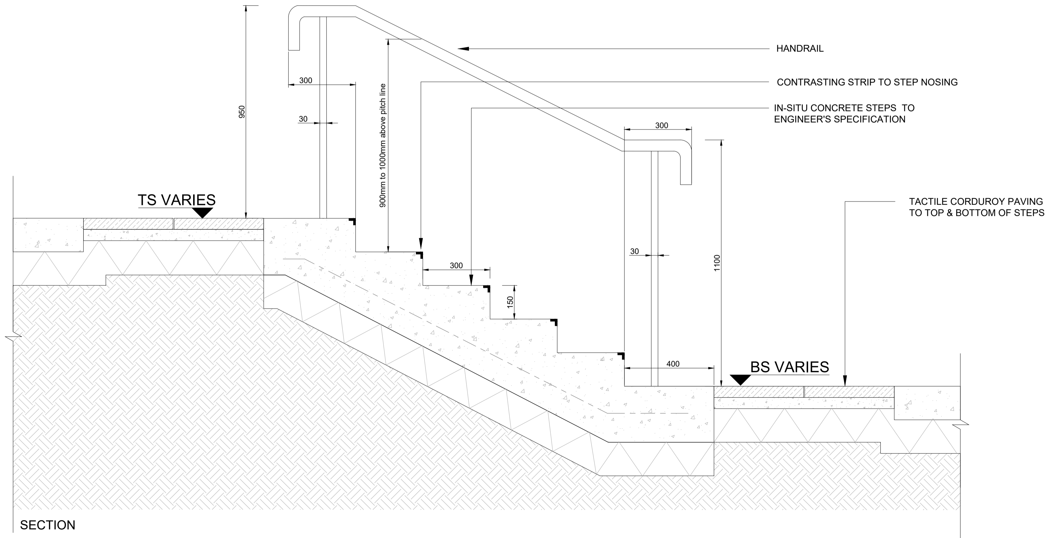
02 TYPICAL DETAIL: IN-SITU CONCRETE STEPS SCALE: 1:10@A1
